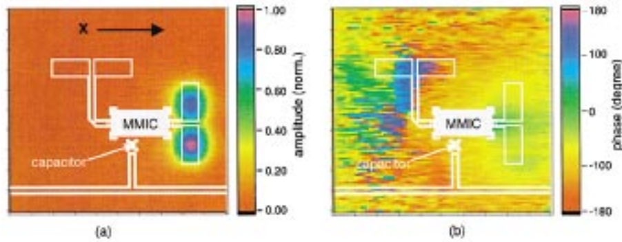
Fig. 7. Electrooptic scan of a unit cell in array B . (a) Normalized amplitude and (b) phase (in degrees). The scan step size is 93\ \mu\text{m} \times 100\ \mu\text{m} , and the scan area is 9.3\ \text{mm} \times 10\ \text{mm} .
