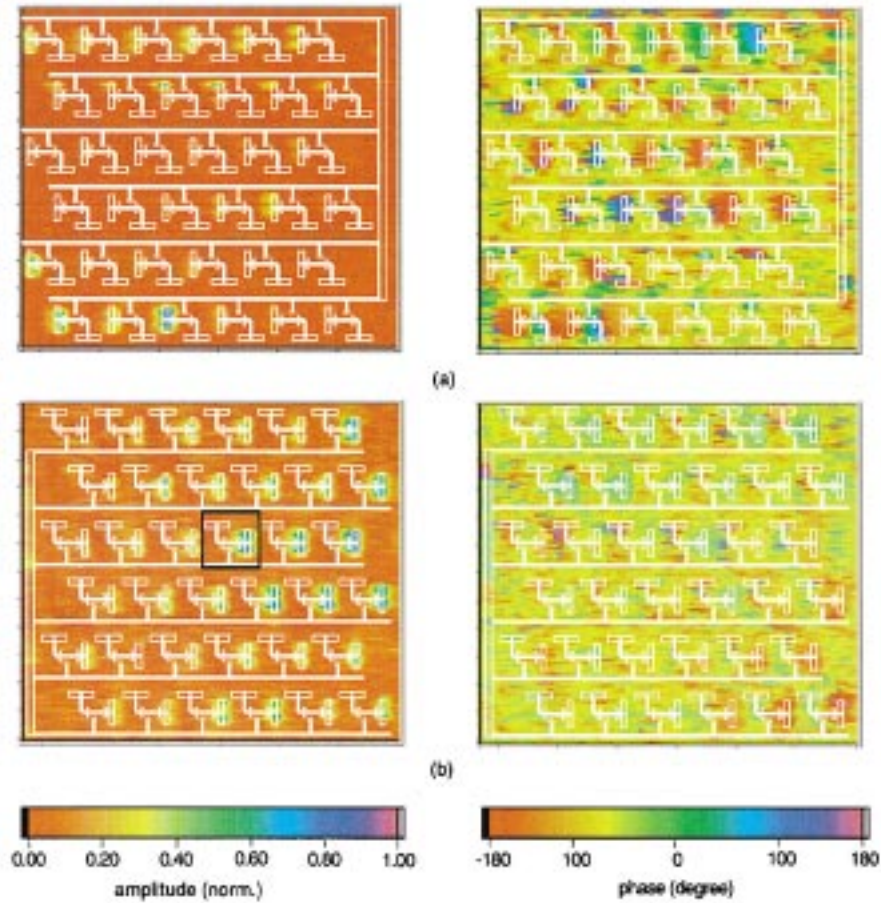
Fig. 8. Amplitude and phase from electrooptic scan of array. (a) Type A . (b) Type B . The square in array B shows the position of the unit cell from Fig. 7. The scan step size is 500\ \mu\text{m} \times 450\ \mu\text{m} , and total scan area is 6.3\ \text{cm} \times 5.4\ \text{cm} .
